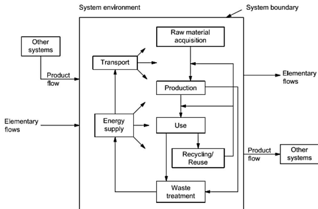
Figure 23 Example of a product system for LCA 106
